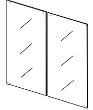
SWINGING GLASS DOOR W/O GLASS LOCK YG 880 760W x 770H x 5THK
