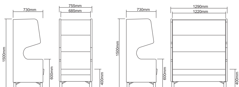
CH-HUME-01 755W x 730D x 1500H mm
